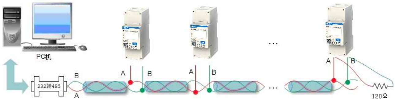
Figure 4 Schematic diagram of communication connection
